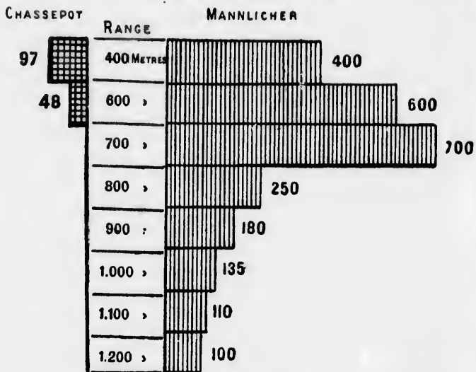
Breadth of Zone of Effective Fire against Cavalry (2 m. 70 cm. in height) at various Ranges
